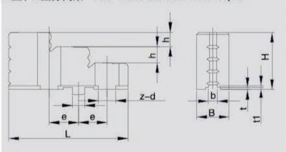
A型、D型分离爪 Two-Piece Jaws for Form A, D
