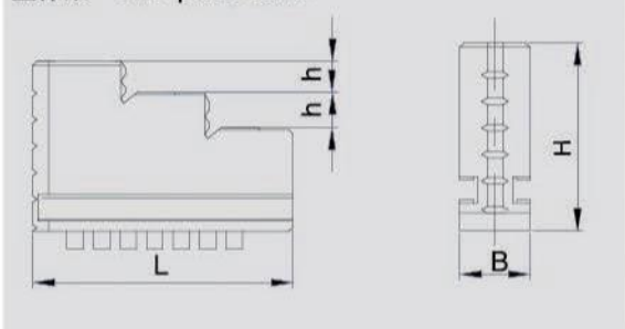
整体爪 One-piece Jaws
